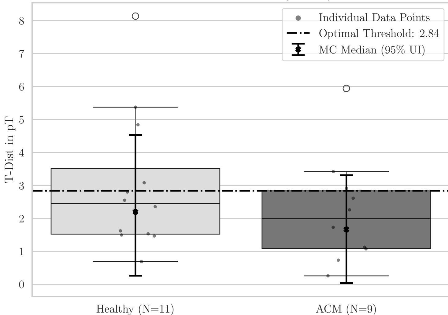
Box Plot for ST T-Dist (NL YZ)
