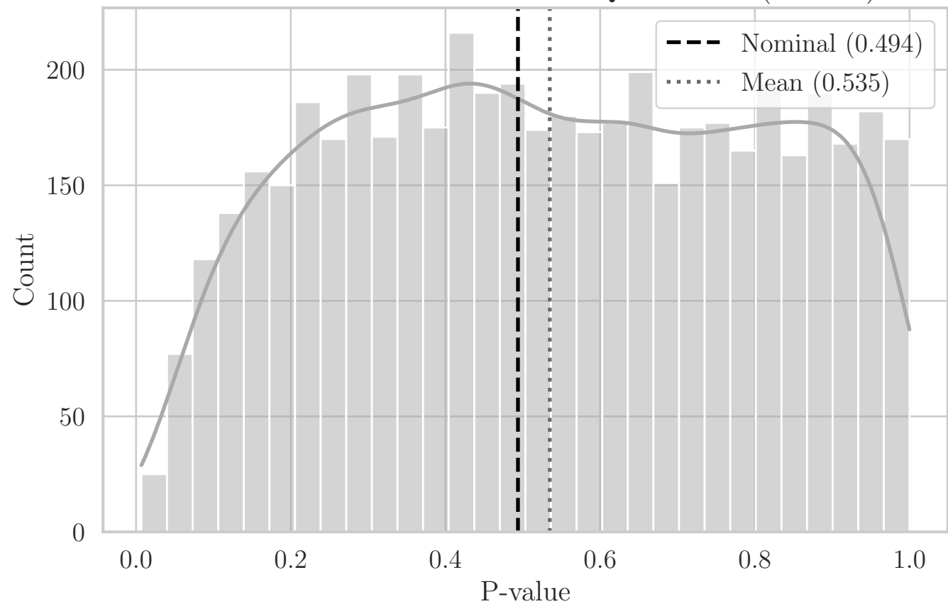
MC Distribution of P-values for QRS T-Dist (OT YZ)
