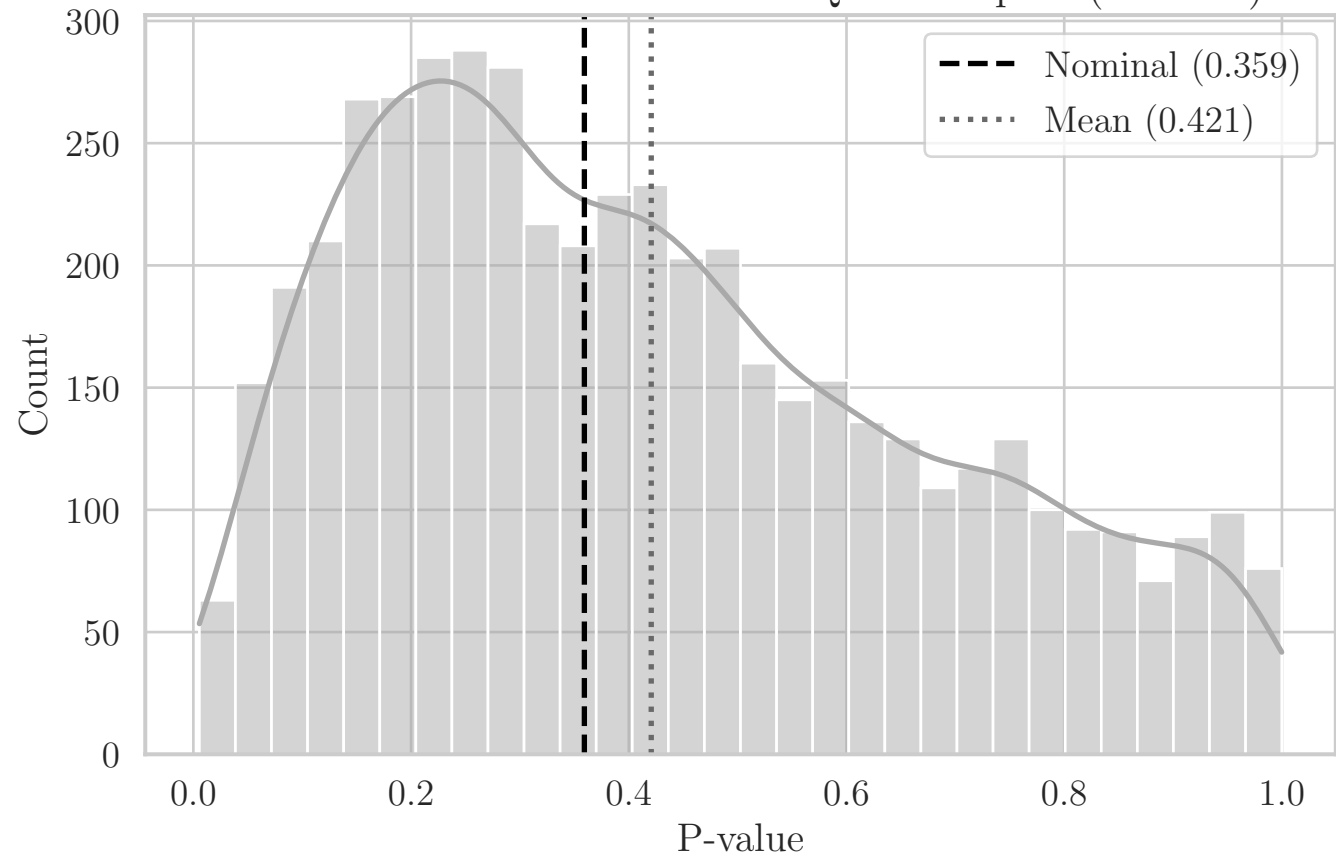
MC Distribution of P-values for QRS Compact (OW YZ)
