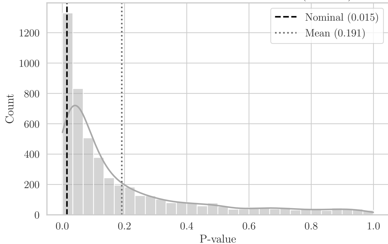
MC Distribution of P-values for ST Area (OW YZ)
