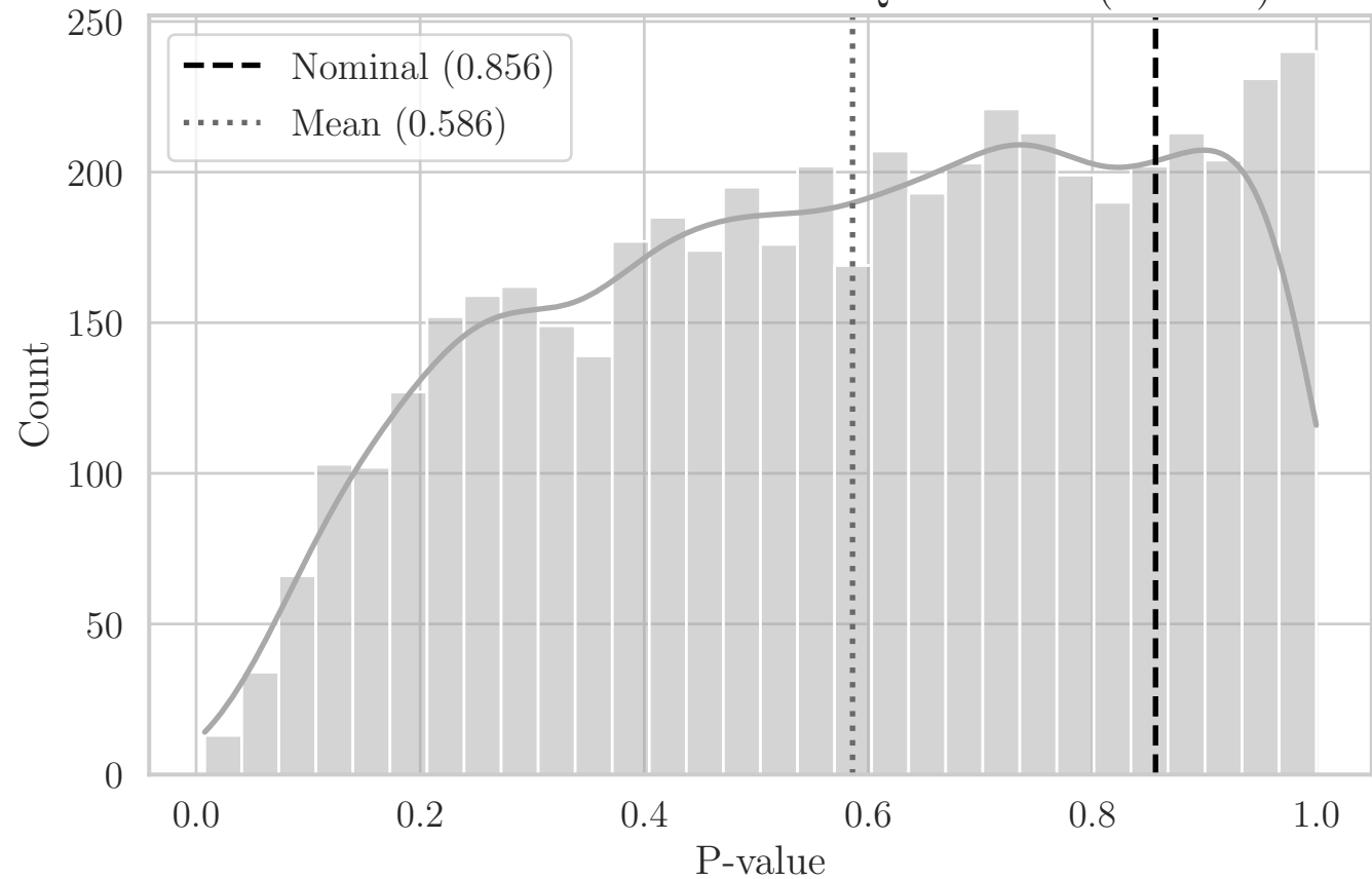
MC Distribution of P-values for QRS T-Dist (OX XY)
