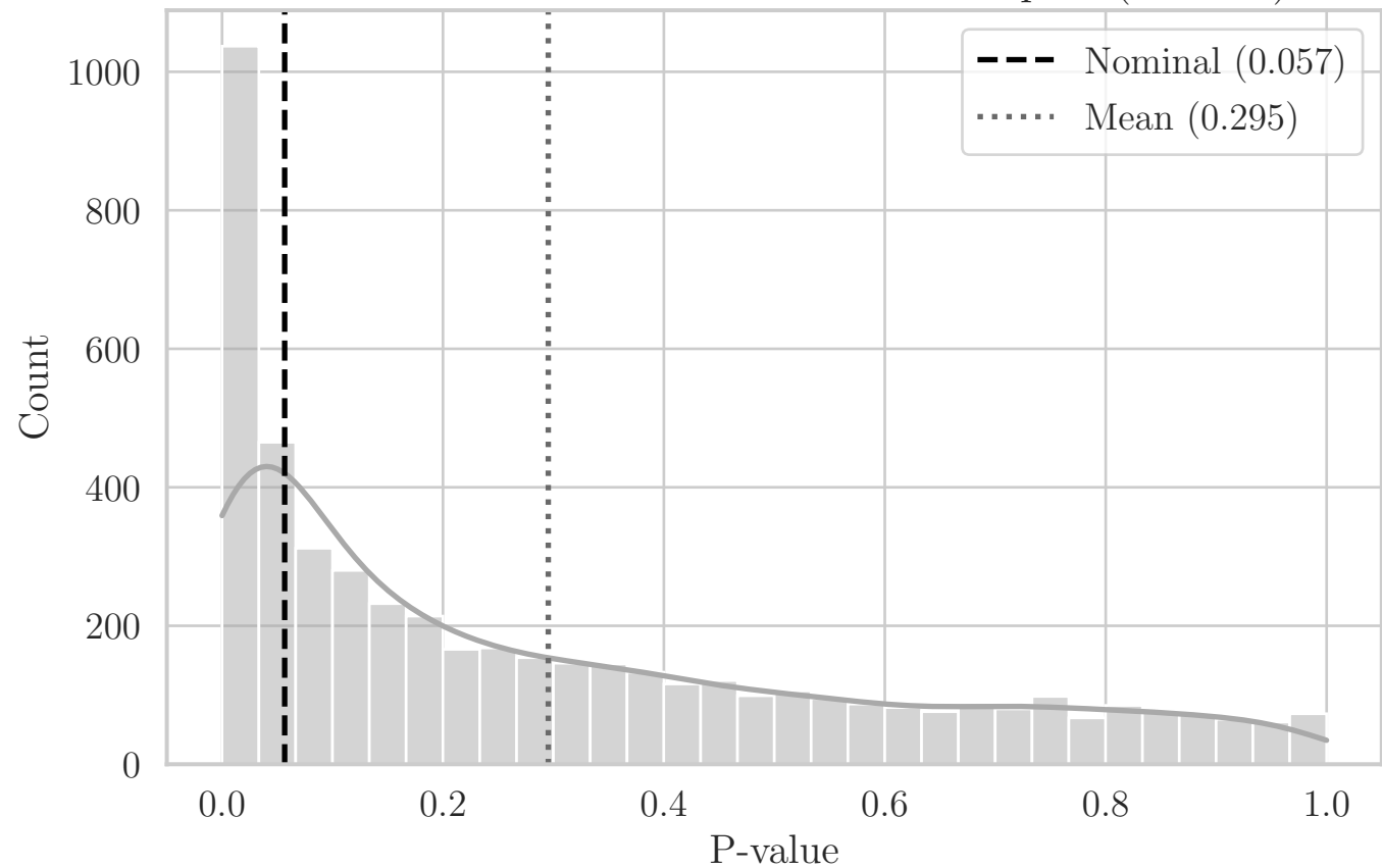
MC Distribution of P-values for ST Compact (OY XY)
