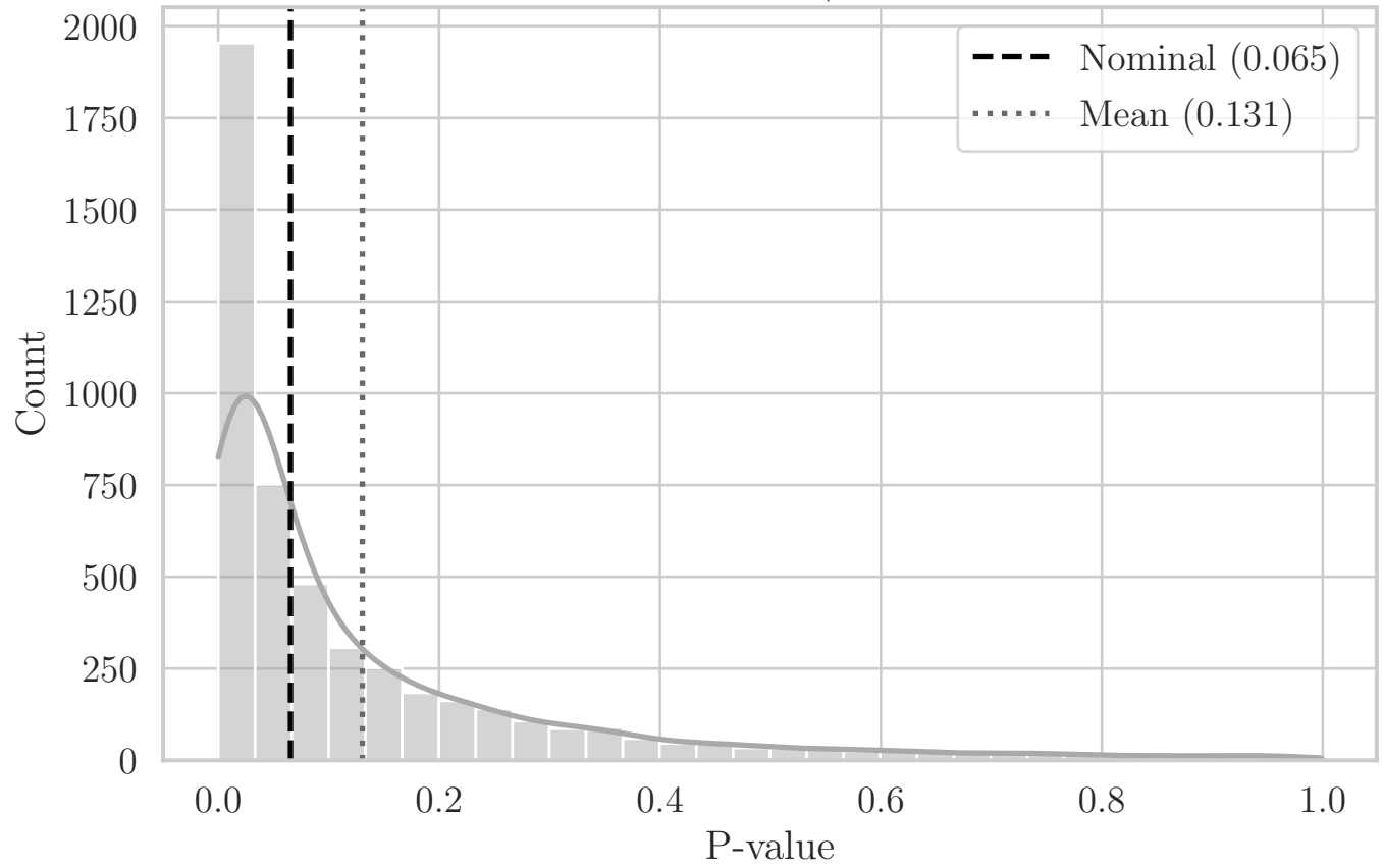
MC Distribution of P-values for QRS T-Dist (Aggregated Bottom-Left Quadrant YZ)
