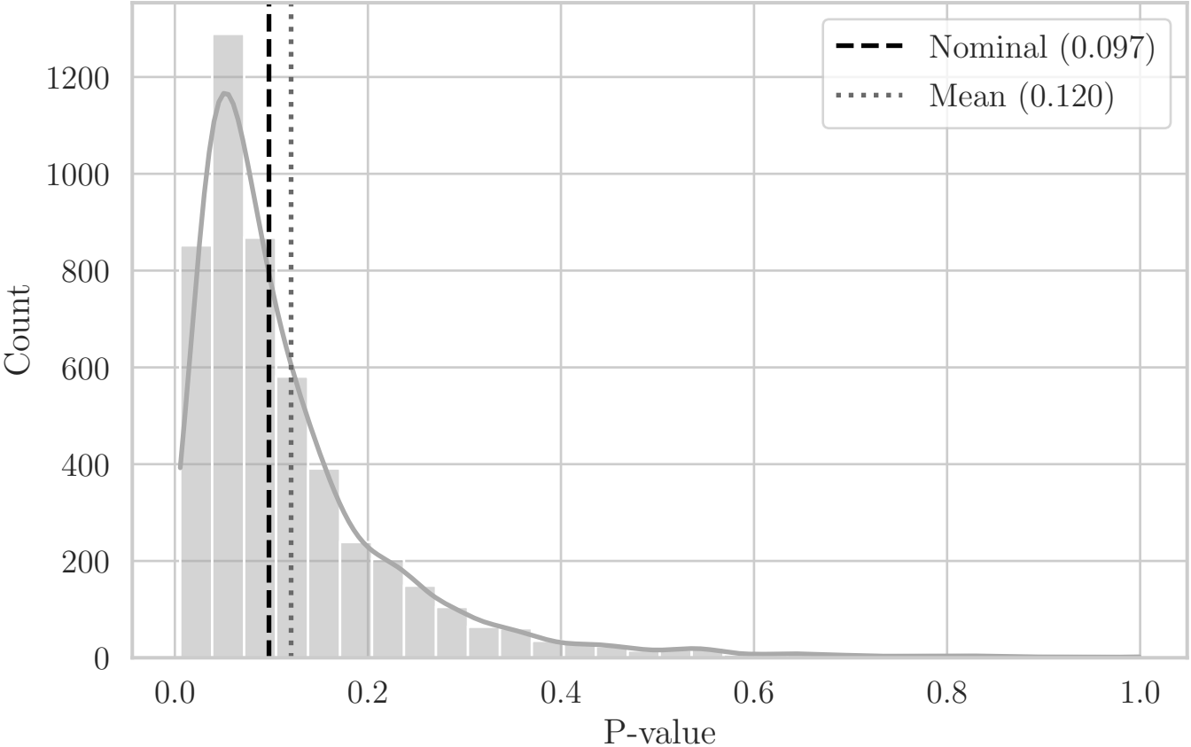
MC Distribution of P-values for QRS Area (Aggregated Bottom-Right Quadrant YZ)
