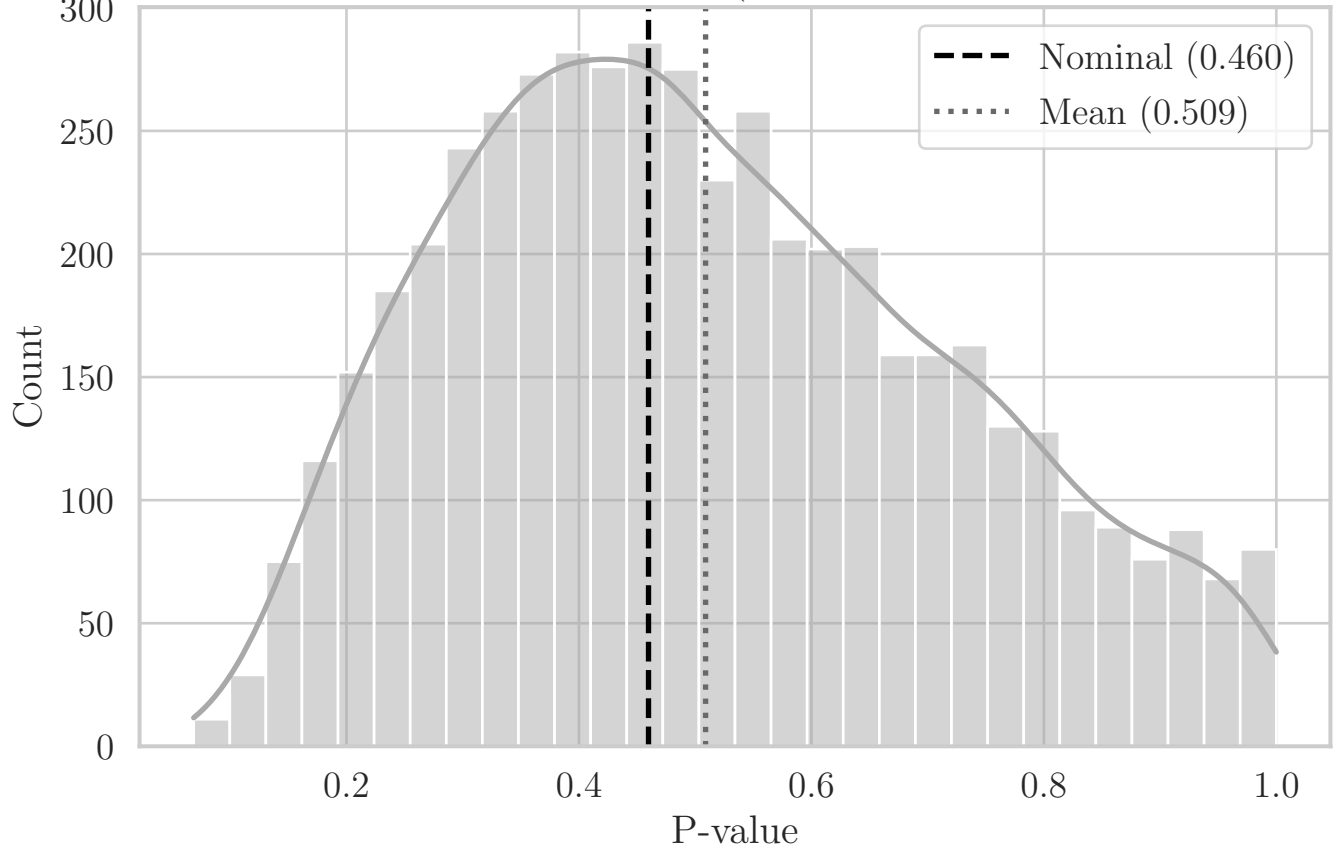
MC Distribution of P-values for T Angle (Aggregated Bottom-Right Quadrant YZ)
