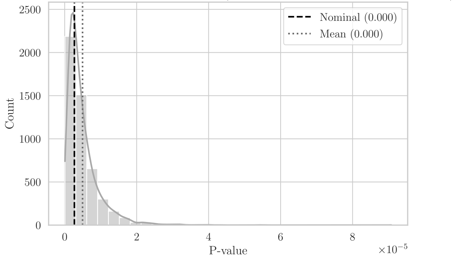
MC Distribution of P-values for T Area (Aggregated Bottom-Right Quadrant YZ)
