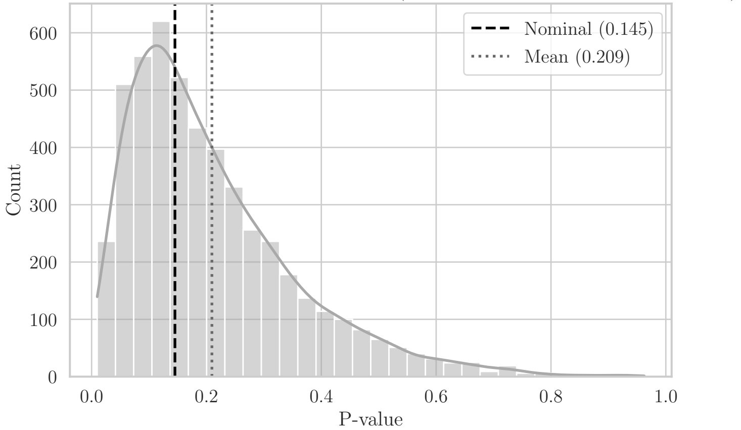
MC Distribution of P-values for ST Angle (Aggregated Top-Left Quadrant XY)
