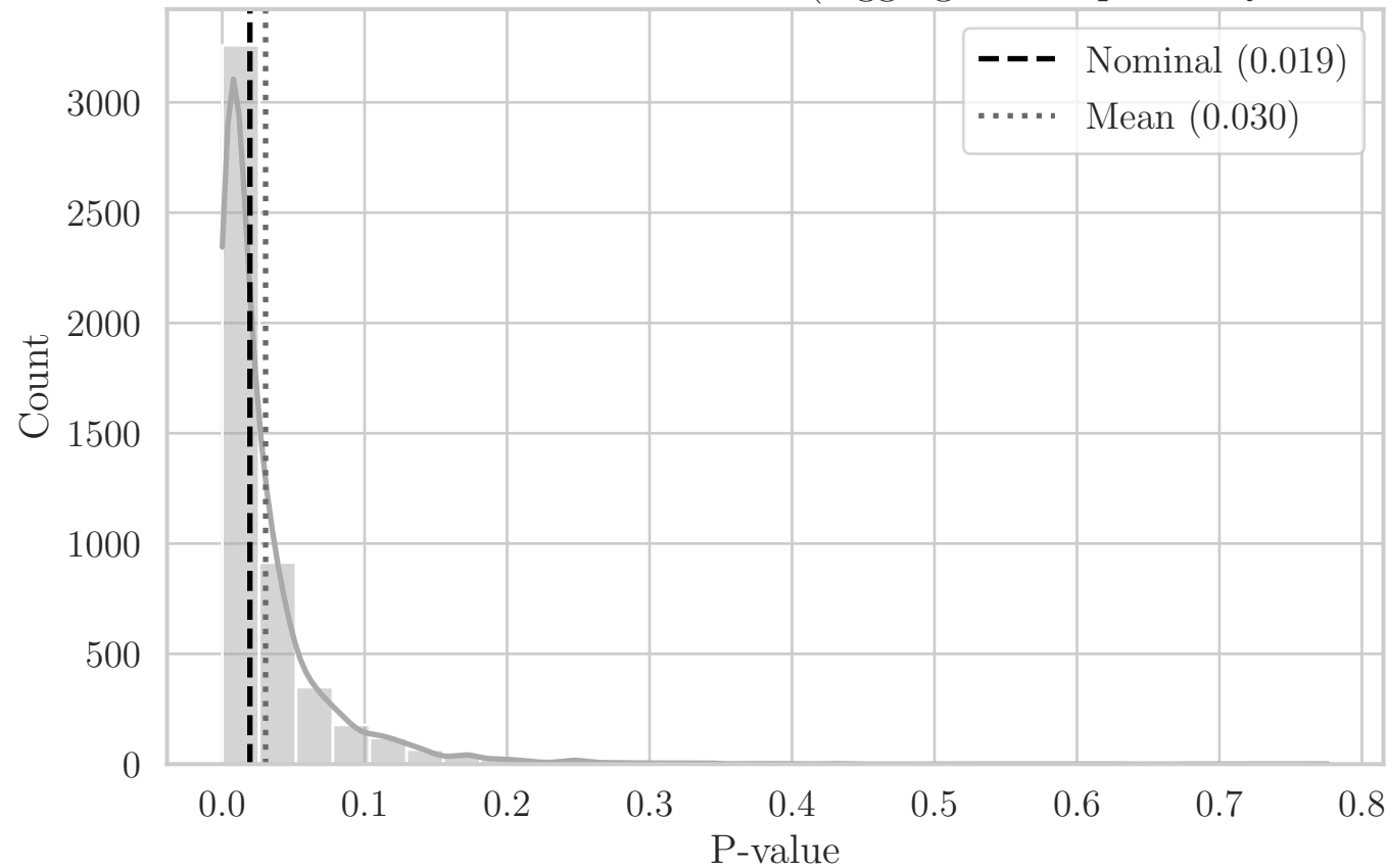
MC Distribution of P-values for T Area (Aggregated Top-Left Quadrant XY)
