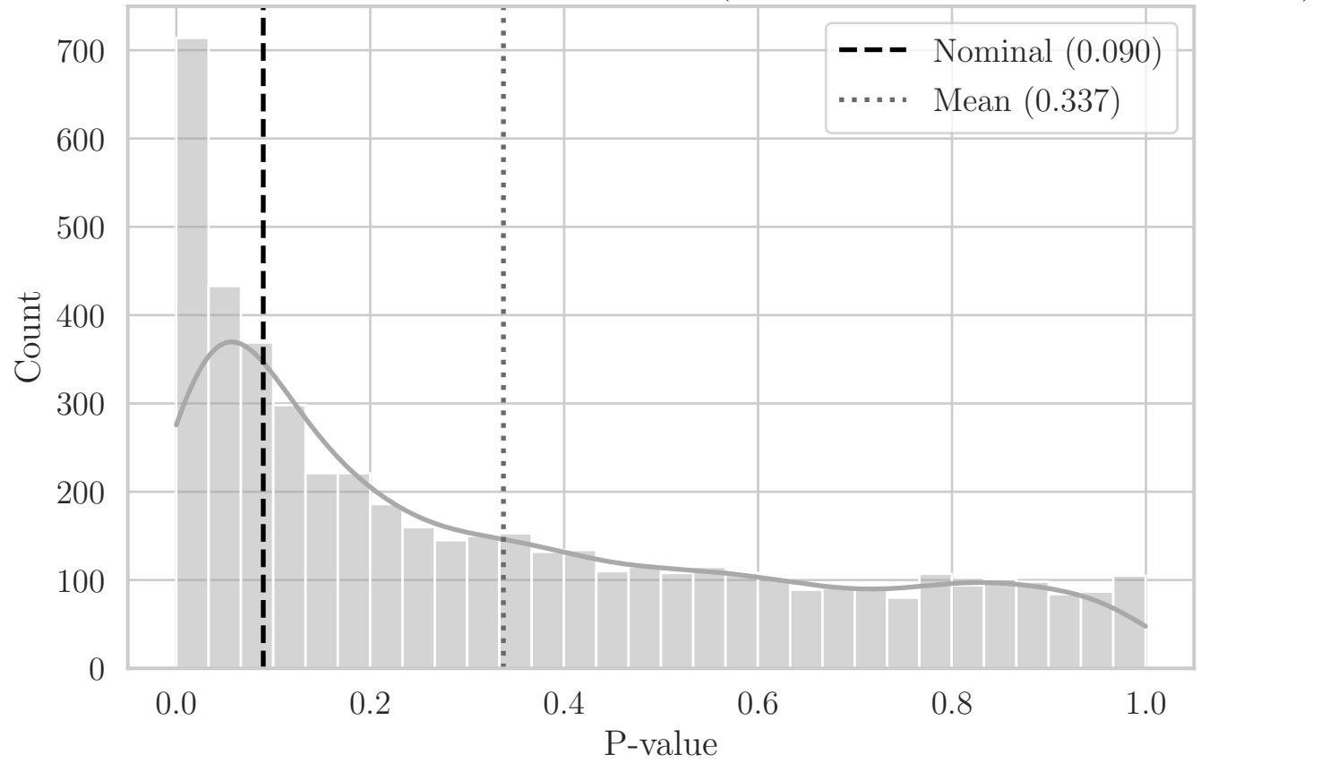
MC Distribution of P-values for ST T-Dist (Aggregated Top-Left Quadrant YZ)
