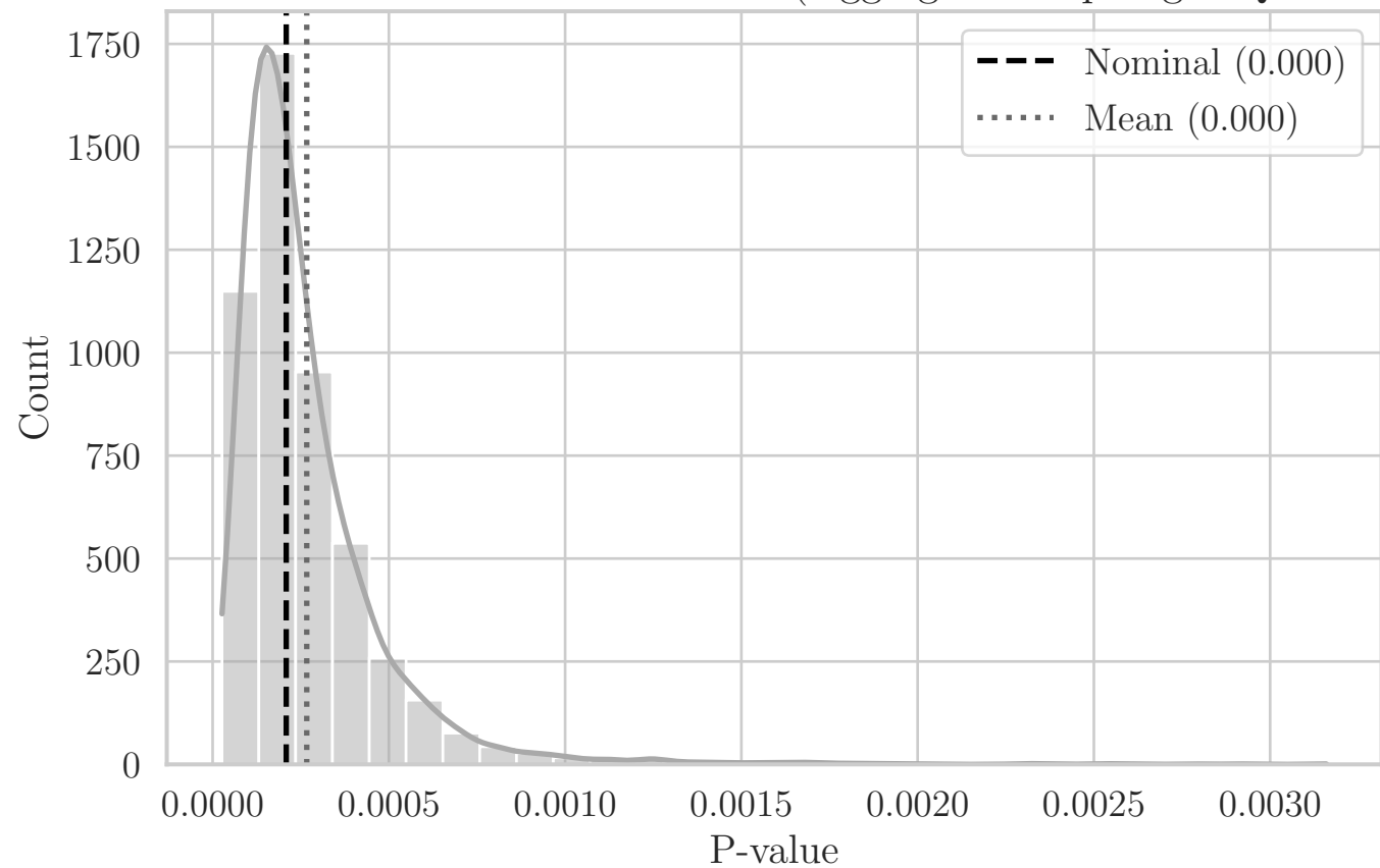
MC Distribution of P-values for T Area (Aggregated Top-Right Quadrant XY)
