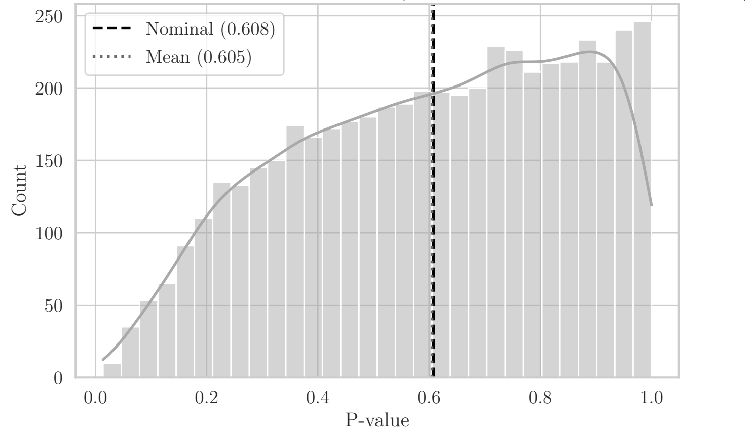
MC Distribution of P-values for ST Angle (Aggregated Top-Right Quadrant YZ)
