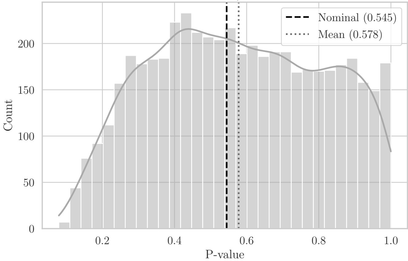
MC Distribution of P-values for T Angle (Aggregated Top-Right Quadrant YZ)
