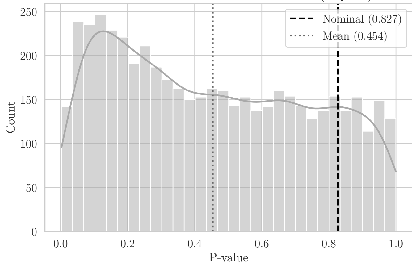
MC Distribution of P-values for ST Area (YQ XY)
