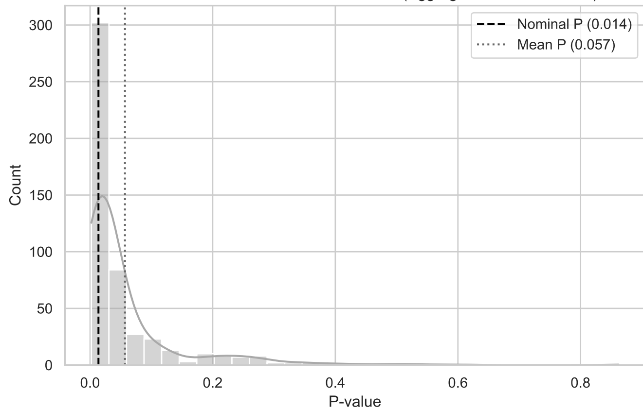
MC Distribution of P-values for QRS Area (Aggregated BottomLeft XY)
