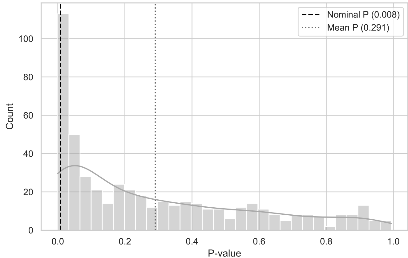
MC Distribution of P-values for ST T-Dist (Aggregated BottomLeft XY)
