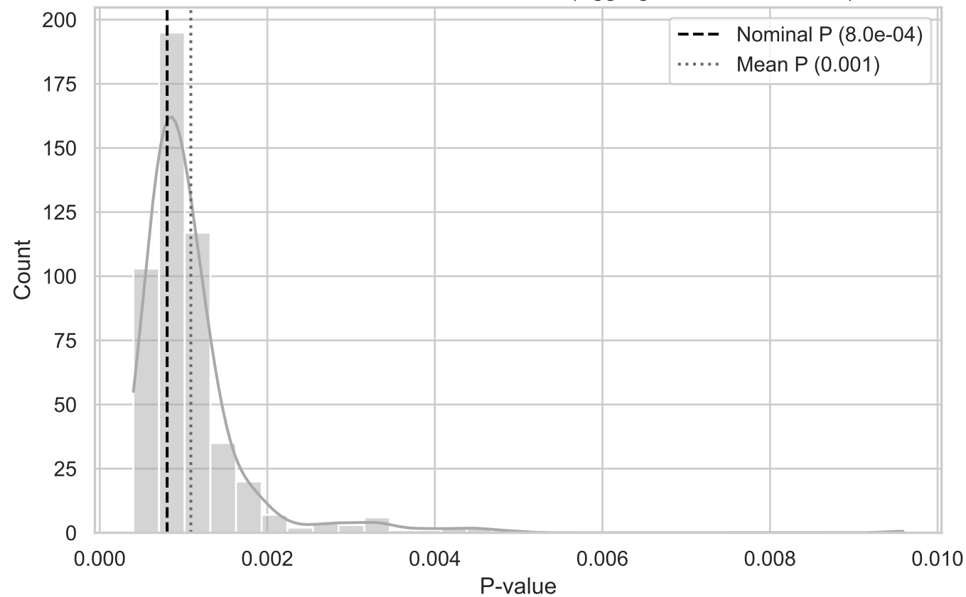
MC Distribution of P-values for T Area (Aggregated BottomLeft XY)
