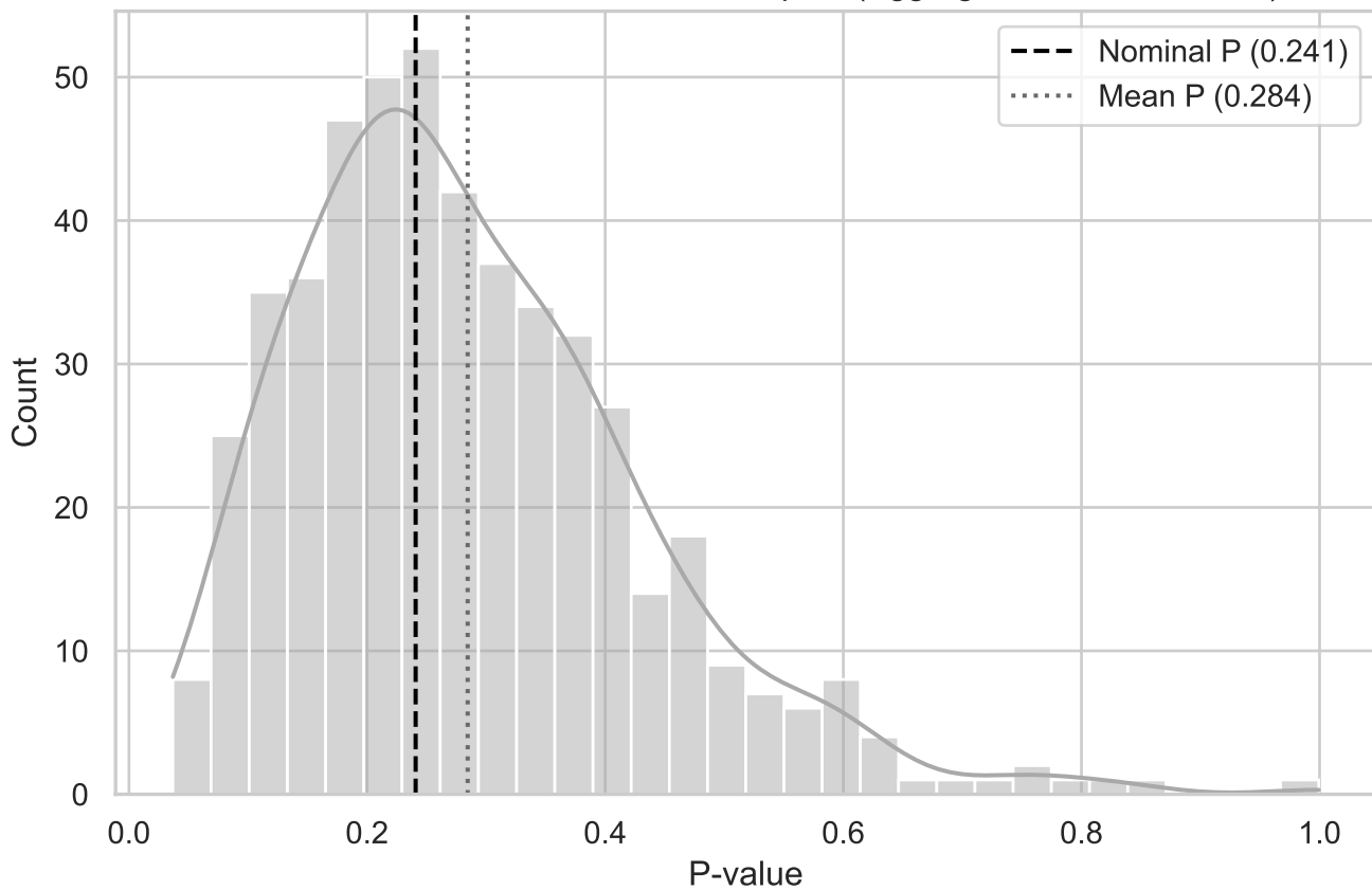
MC Distribution of P-values for T Compact (Aggregated BottomLeft XY)
