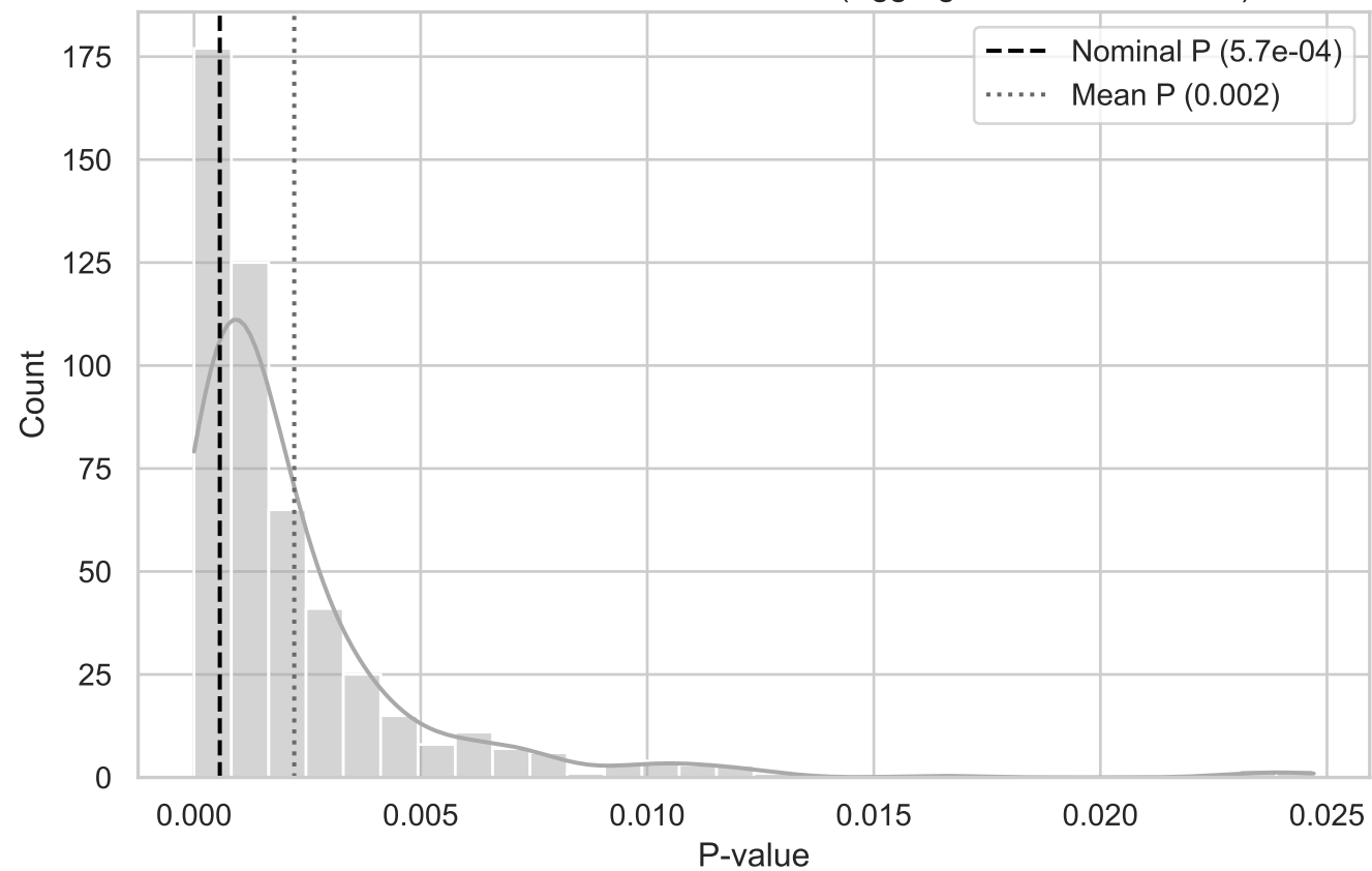
MC Distribution of P-values for T T-Dist (Aggregated BottomLeft YZ)
