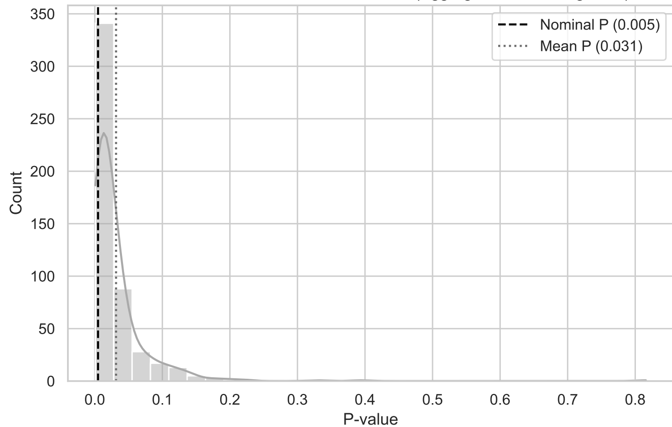
MC Distribution of P-values for QRS Area (Aggregated BottomRight XY)
