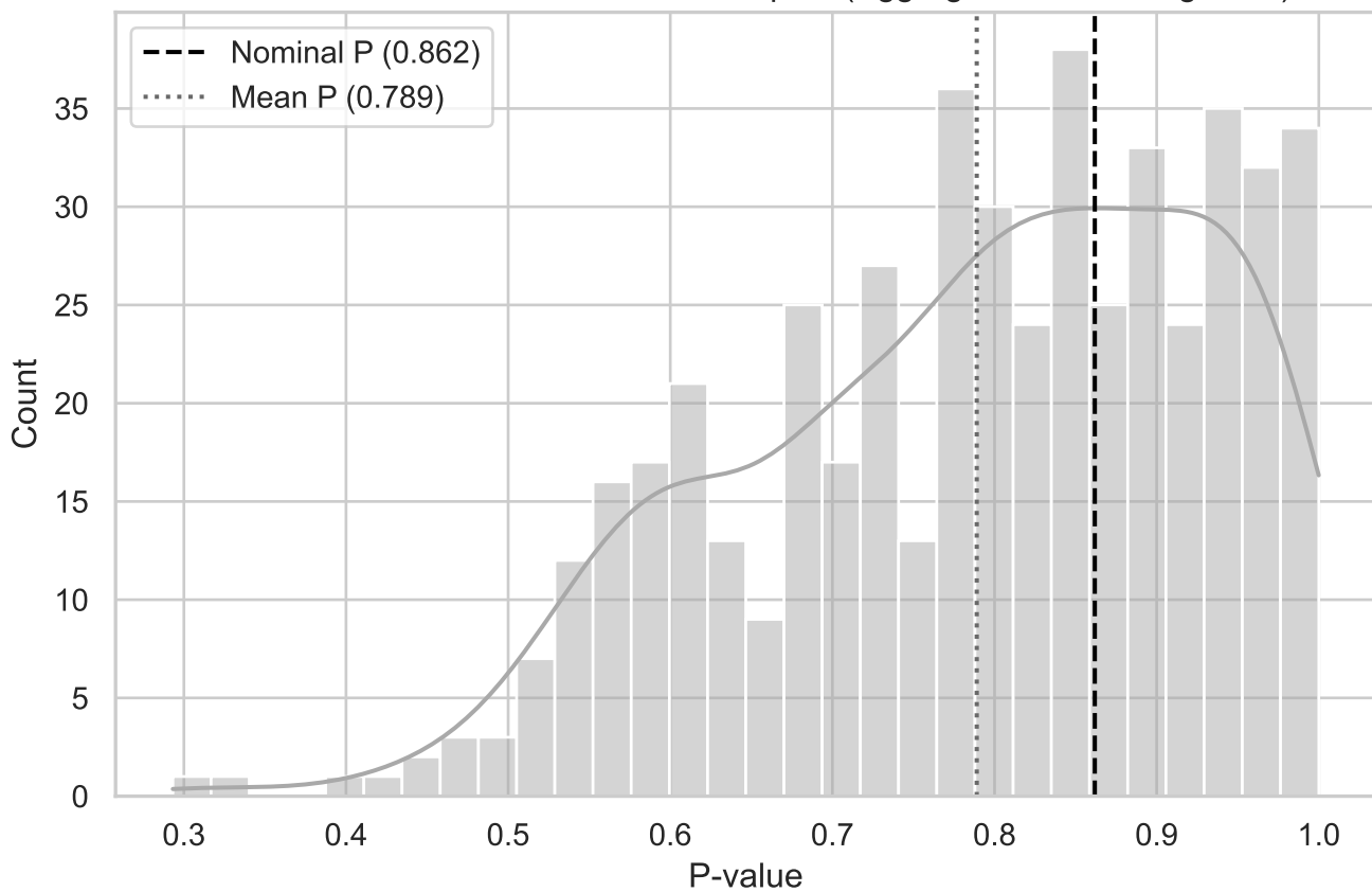
MC Distribution of P-values for T Compact (Aggregated BottomRight XY)
