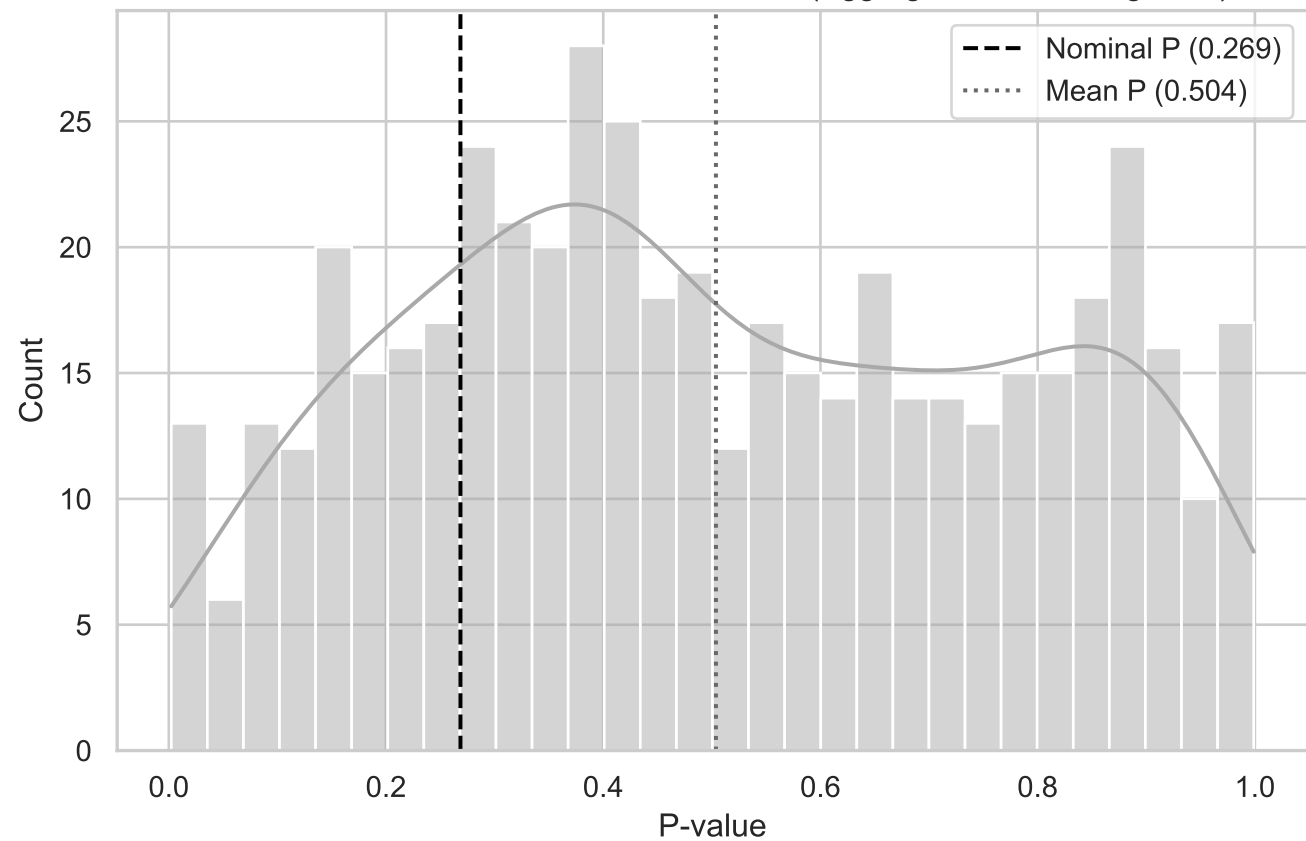
MC Distribution of P-values for QRS T-Dist (Aggregated BottomRight YZ)
