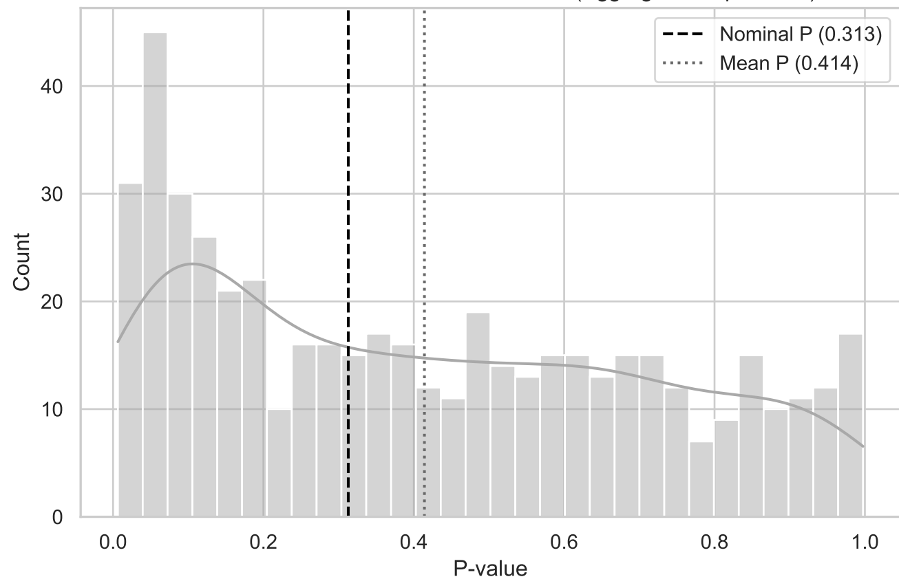
MC Distribution of P-values for QRS Area (Aggregated TopLeft XY)
