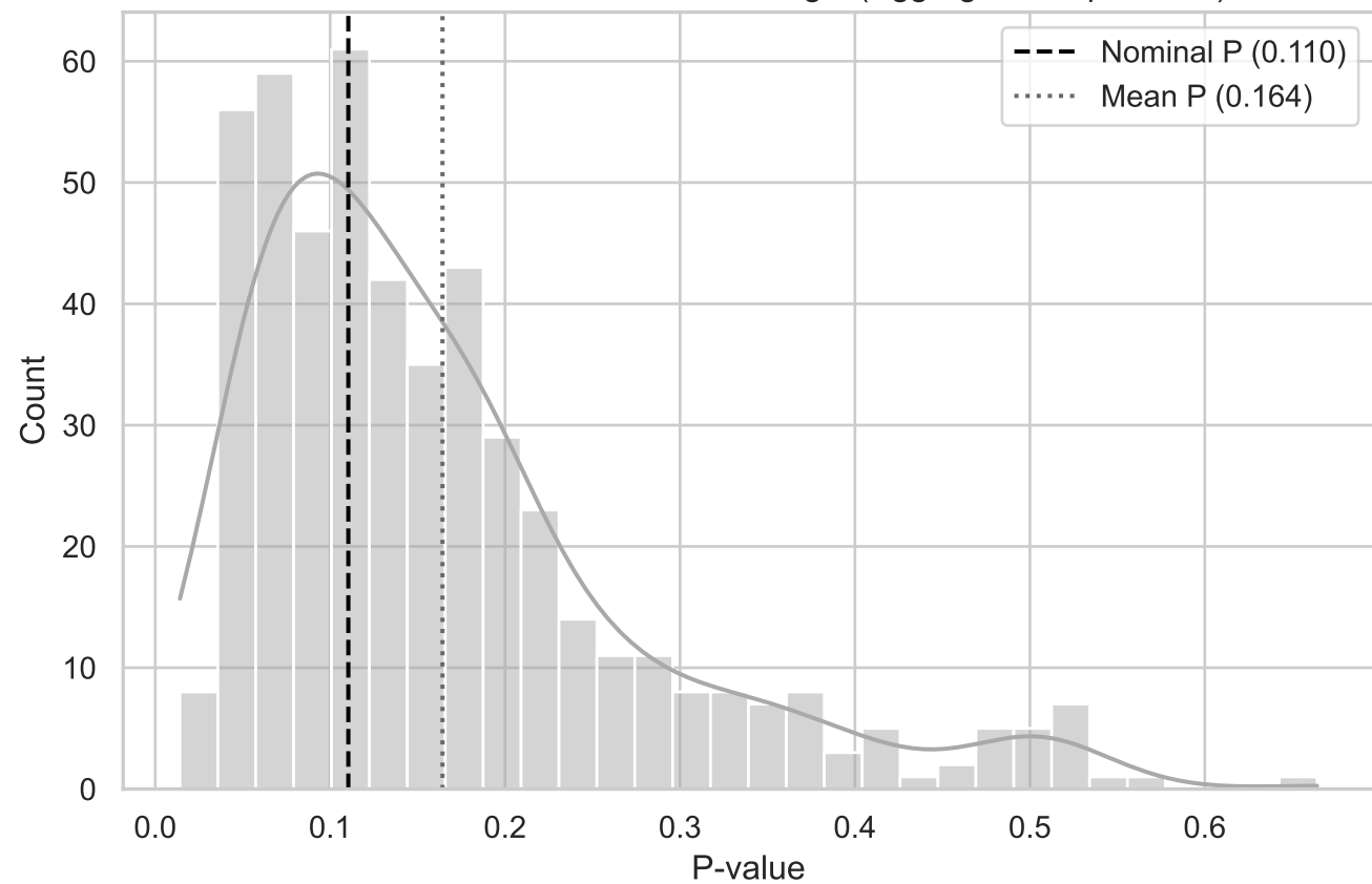
MC Distribution of P-values for T Angle (Aggregated TopLeft XY)
