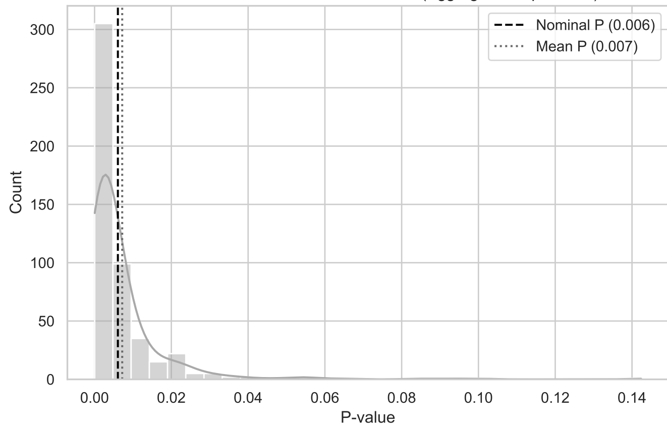
MC Distribution of P-values for T T-Dist (Aggregated TopLeft XY)
