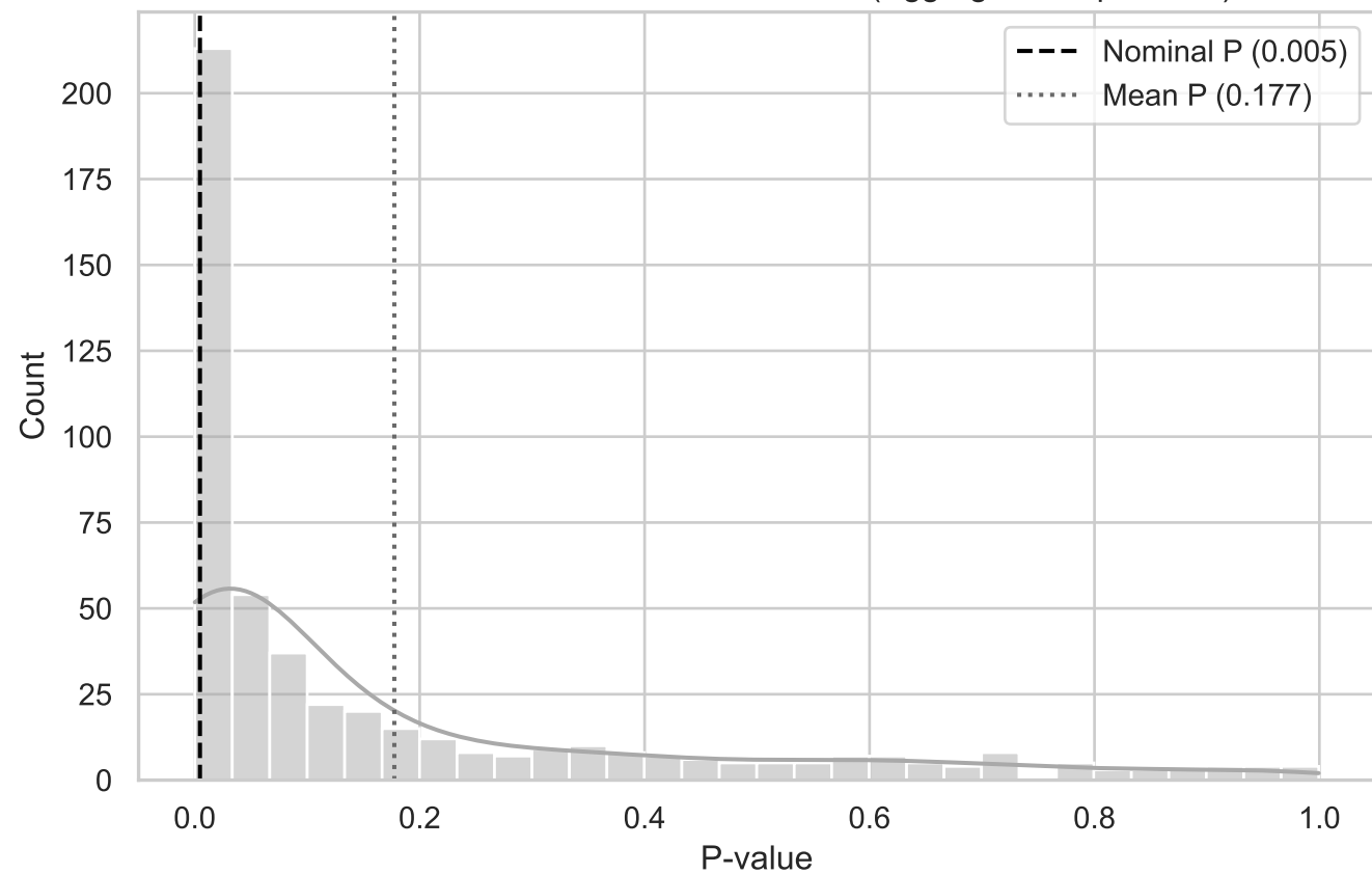
MC Distribution of P-values for ST Area (Aggregated TopLeft YZ)
