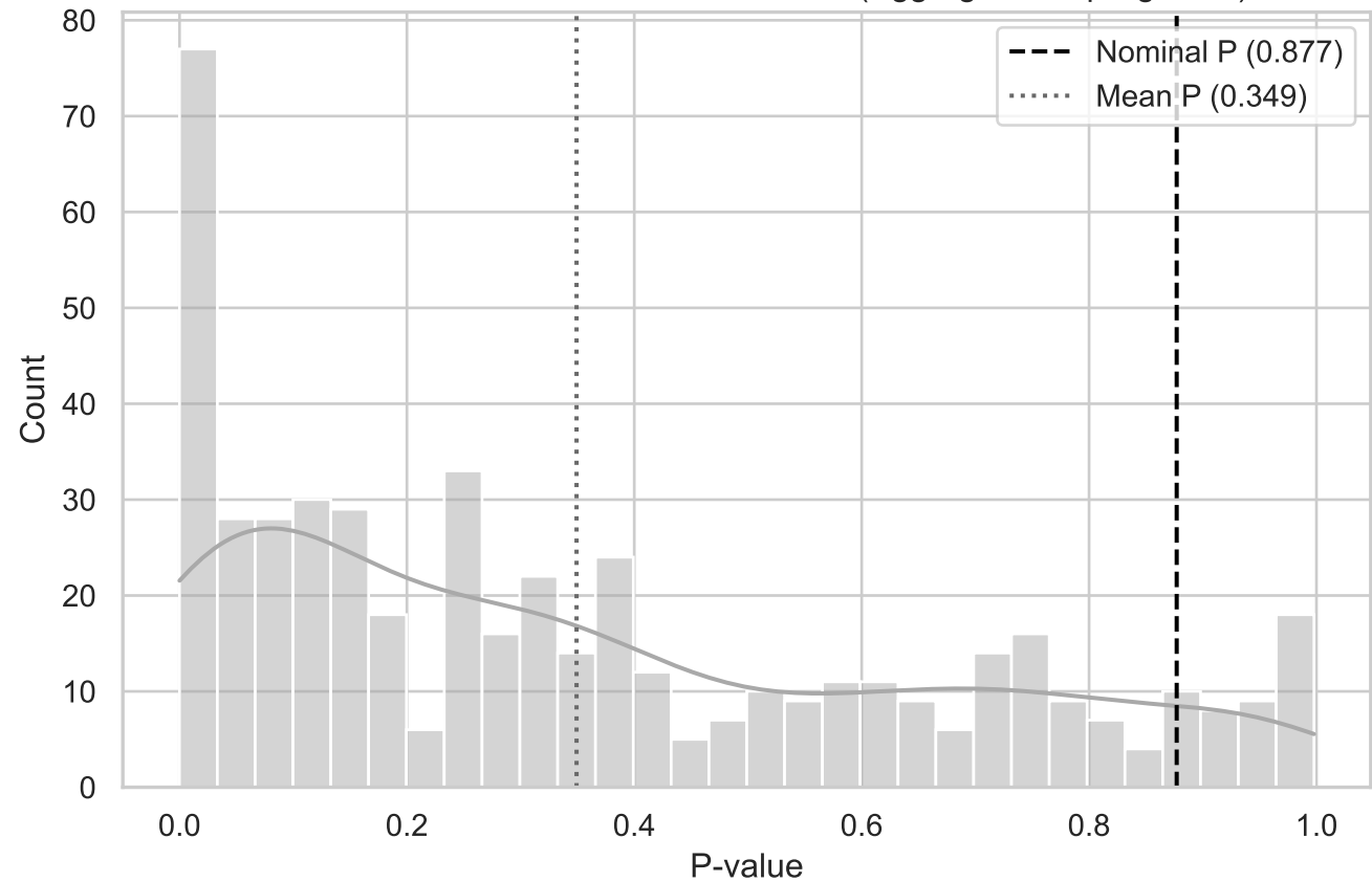
MC Distribution of P-values for ST T-Dist (Aggregated TopRight XY)
