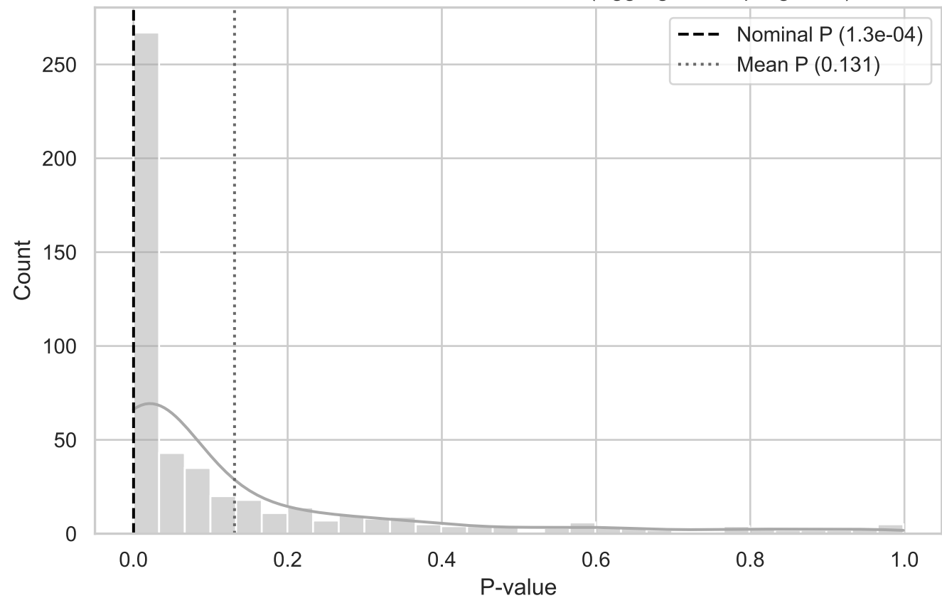
MC Distribution of P-values for ST Area (Aggregated TopRight YZ)
