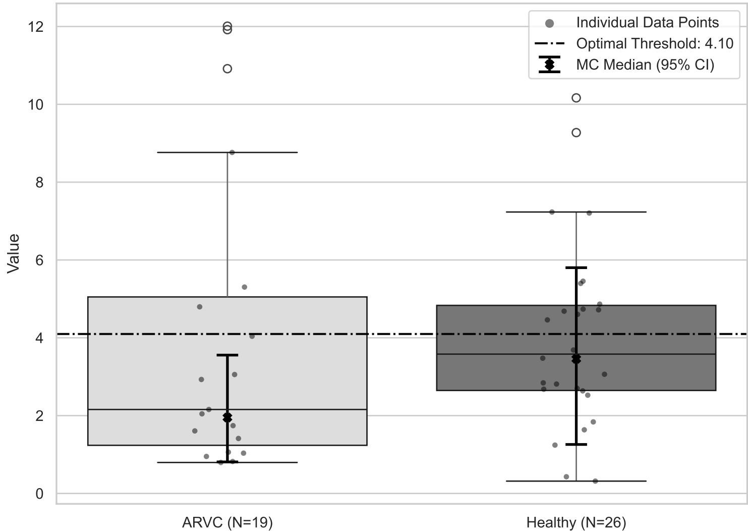
Box Plot of Nominal Data with MC Medians for ST T-Dist (Aggregated TopRight YZ)
