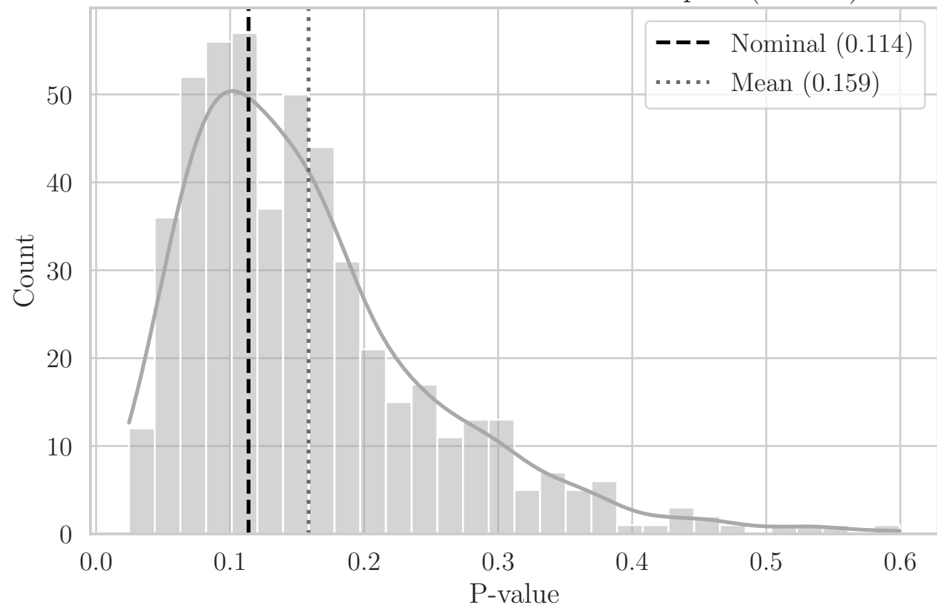
MC Distribution of P-values for T Compact (EZ YZ)
