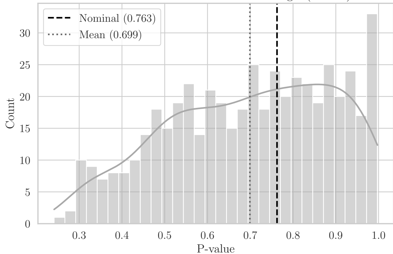
MC Distribution of P-values for T Angle (F0 YZ)
