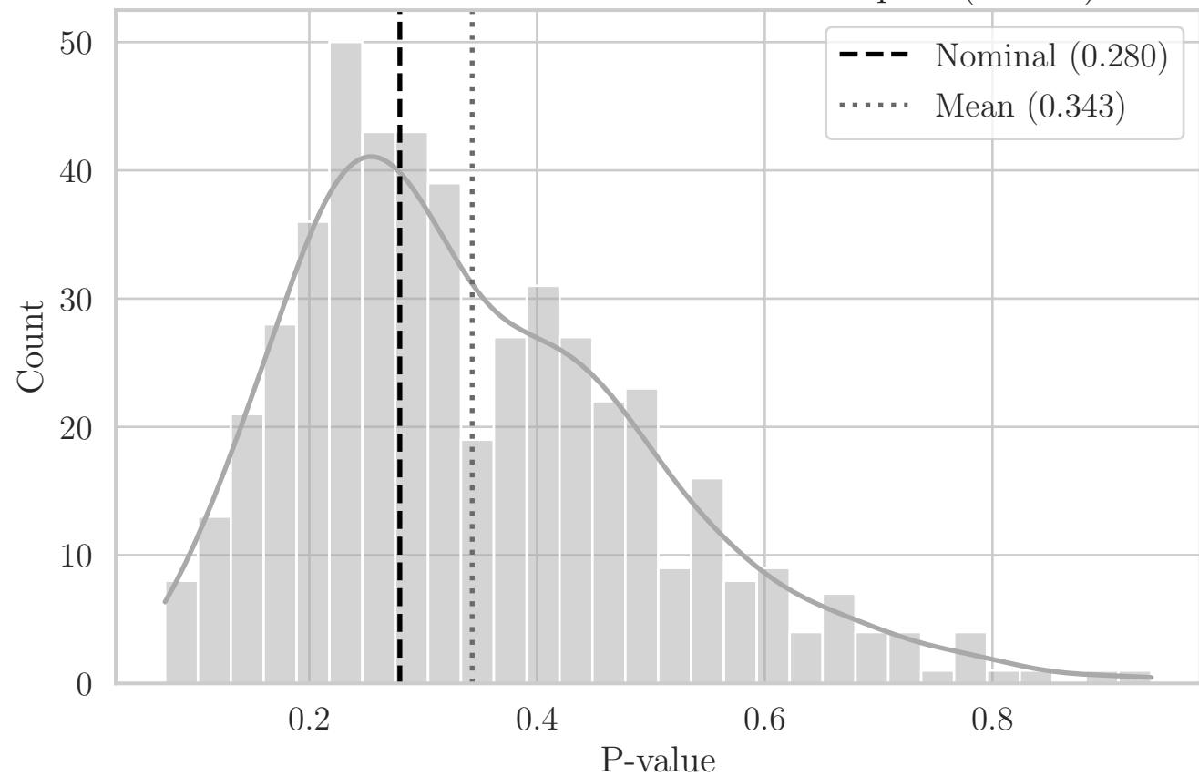
MC Distribution of P-values for T Compact (F1 YZ)
