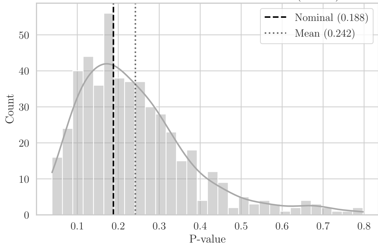
MC Distribution of P-values for T T-Dist (F1 YZ)
