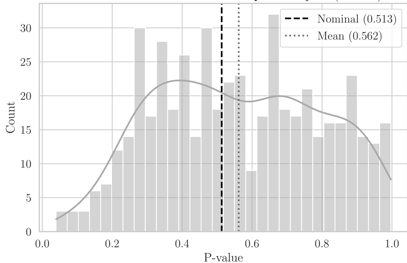
MC Distribution of P-values for QRS Compact (F2 XY)
