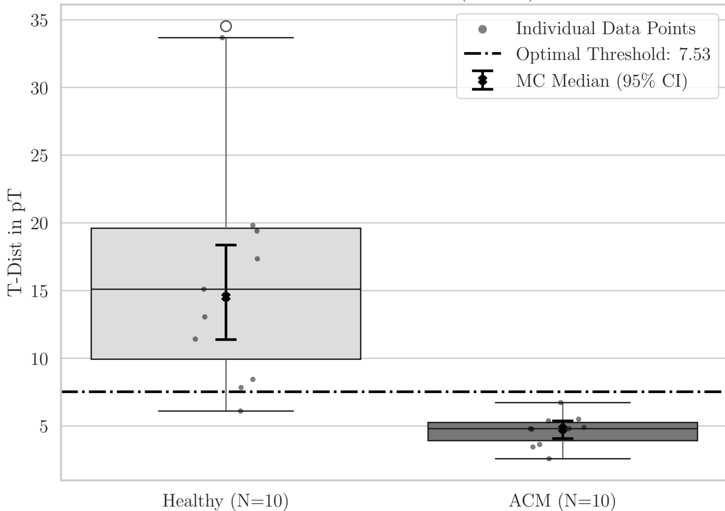
Box Plot for T T-Dist (F2 XY)
