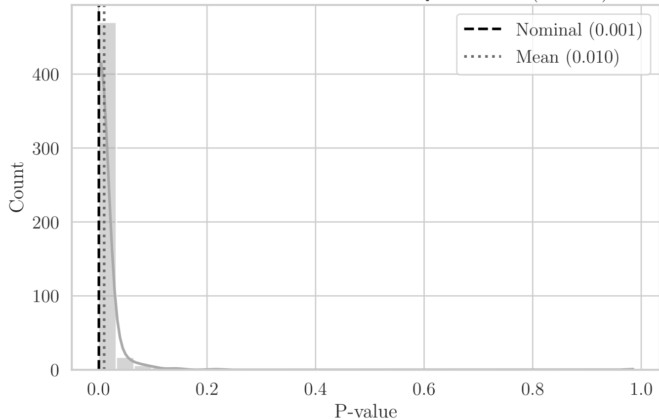
MC Distribution of P-values for QRS T-Dist (NL YZ)
