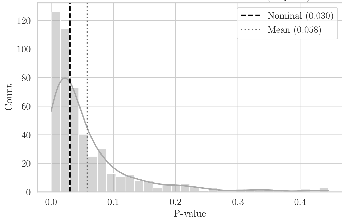
MC Distribution of P-values for T T-Dist (OQ XY)
