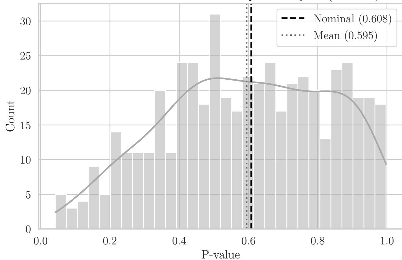
MC Distribution of P-values for QRS Compact (OR XY)
