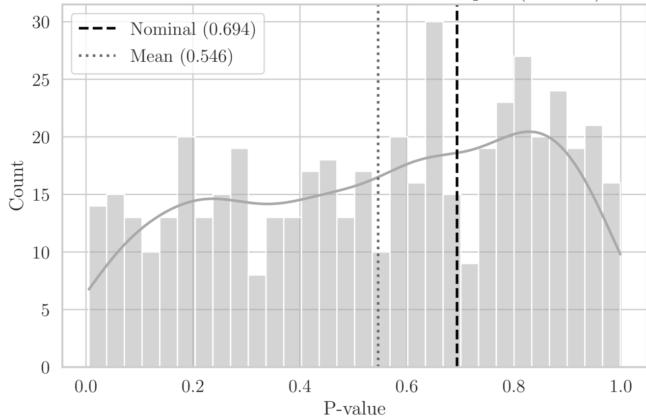
MC Distribution of P-values for ST Compact (OR XY)
