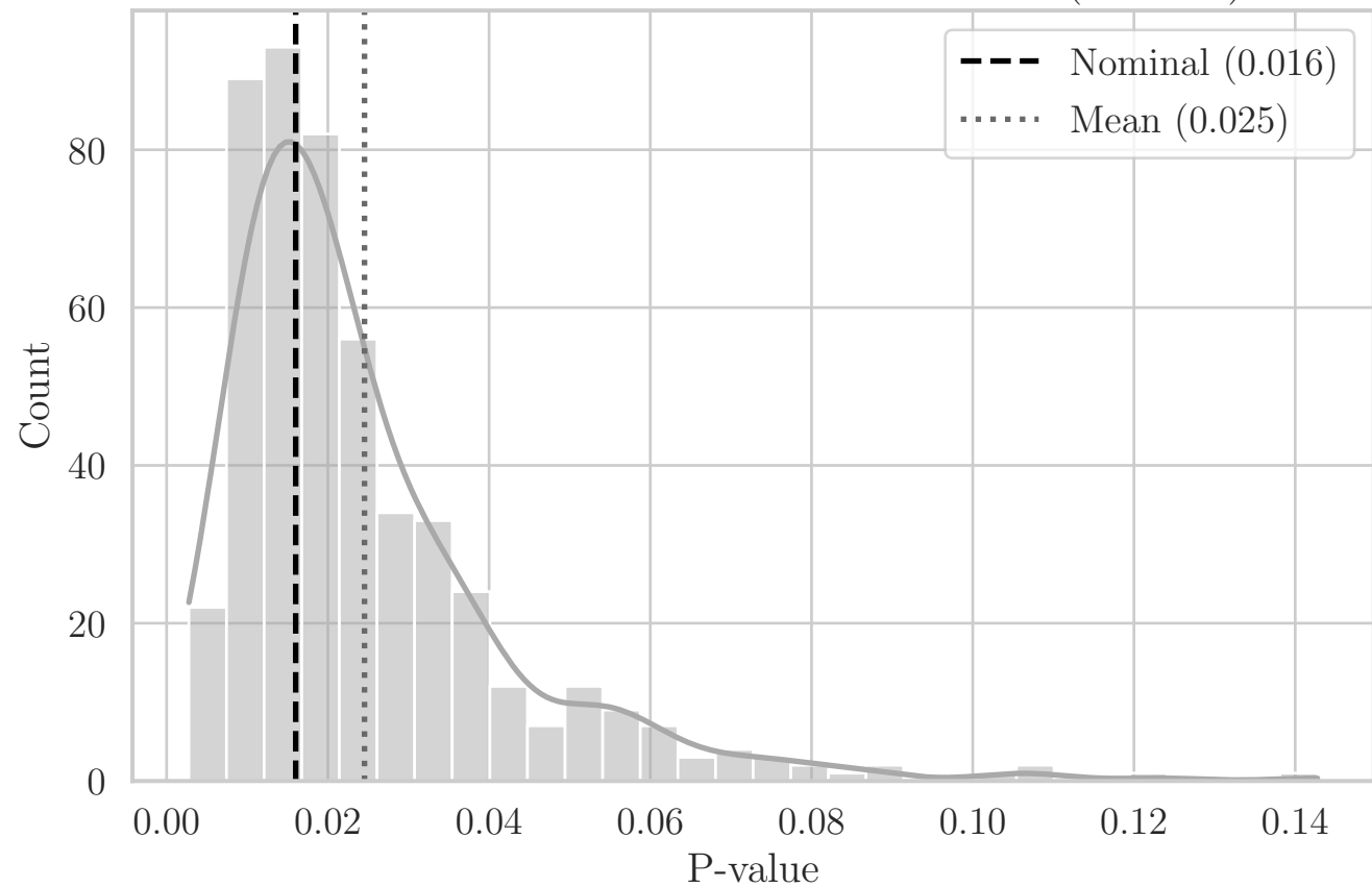
MC Distribution of P-values for T T-Dist (OR XY)
