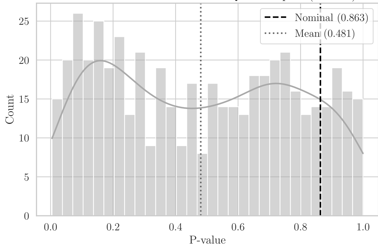
MC Distribution of P-values for QRS Compact (OT YZ)
