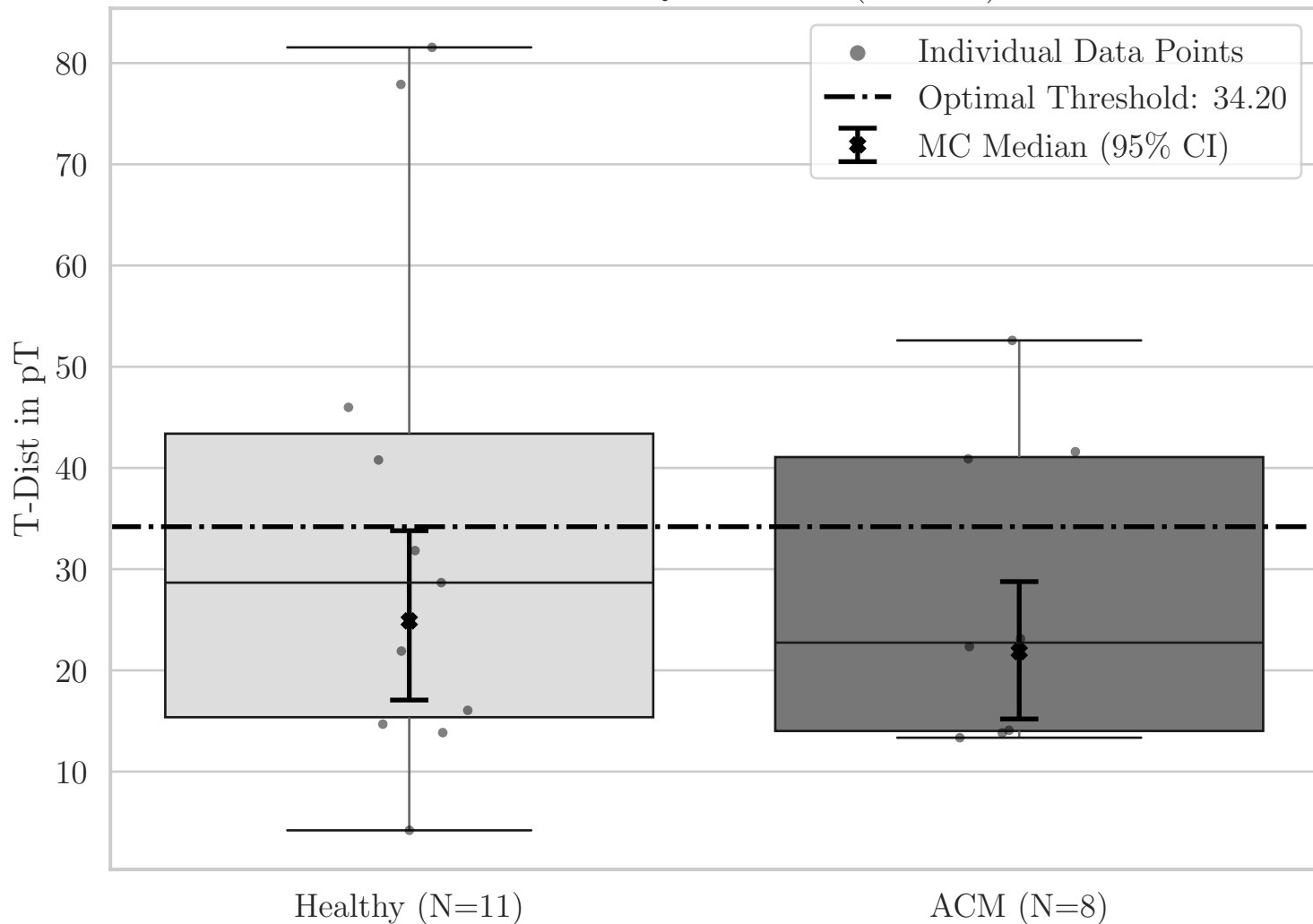
Box Plot for QRS T-Dist (OT YZ)
