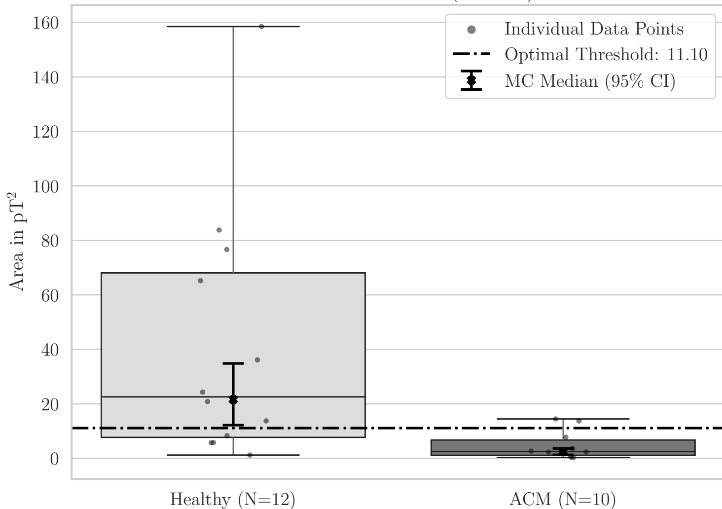
Box Plot for T Area (OY XY)
