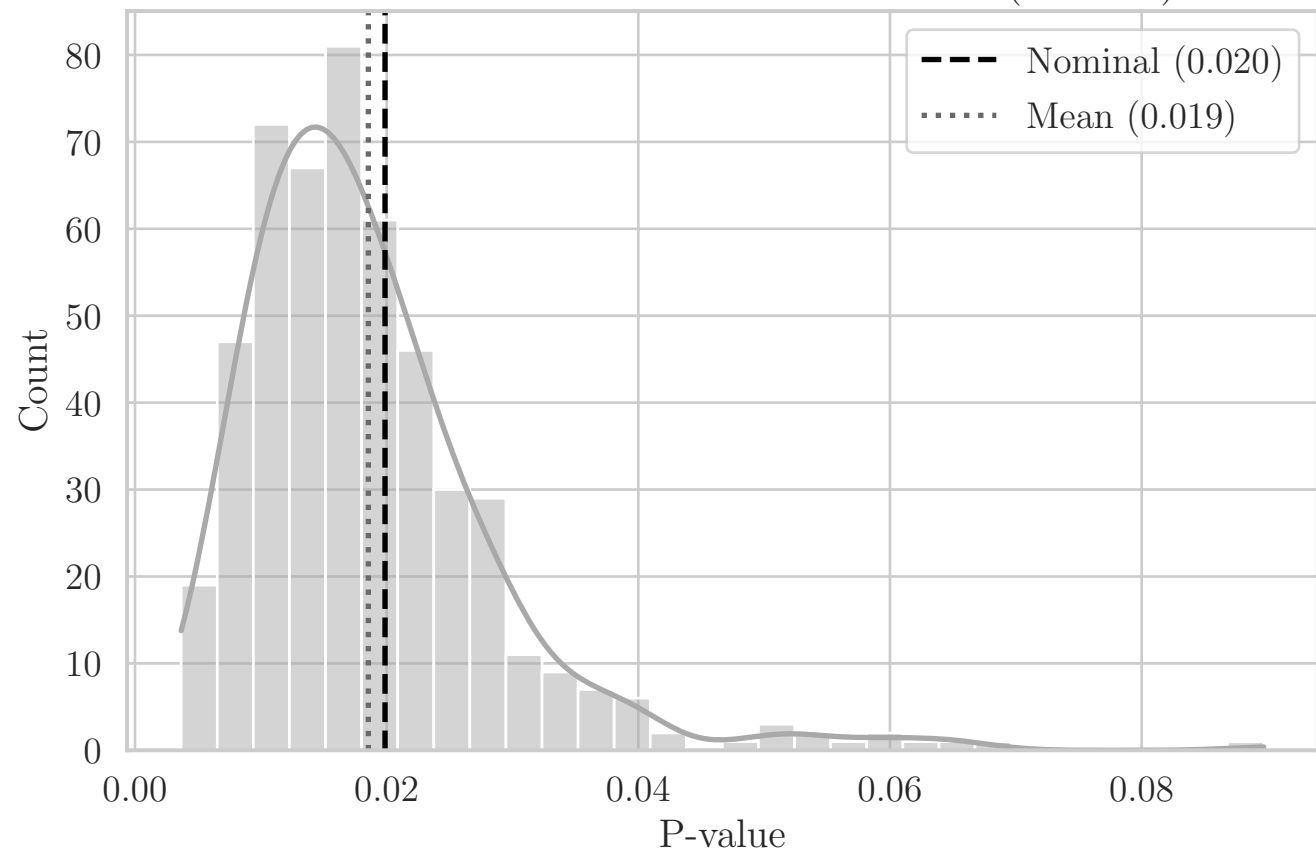
MC Distribution of P-values for T Area (OY XY)
