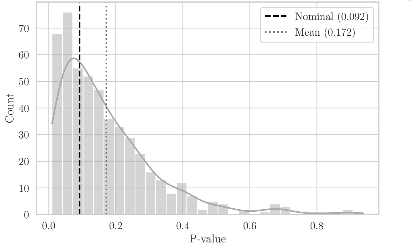
MC Distribution of P-values for T Angle (Aggregated Top-Left Quadrant XY)
