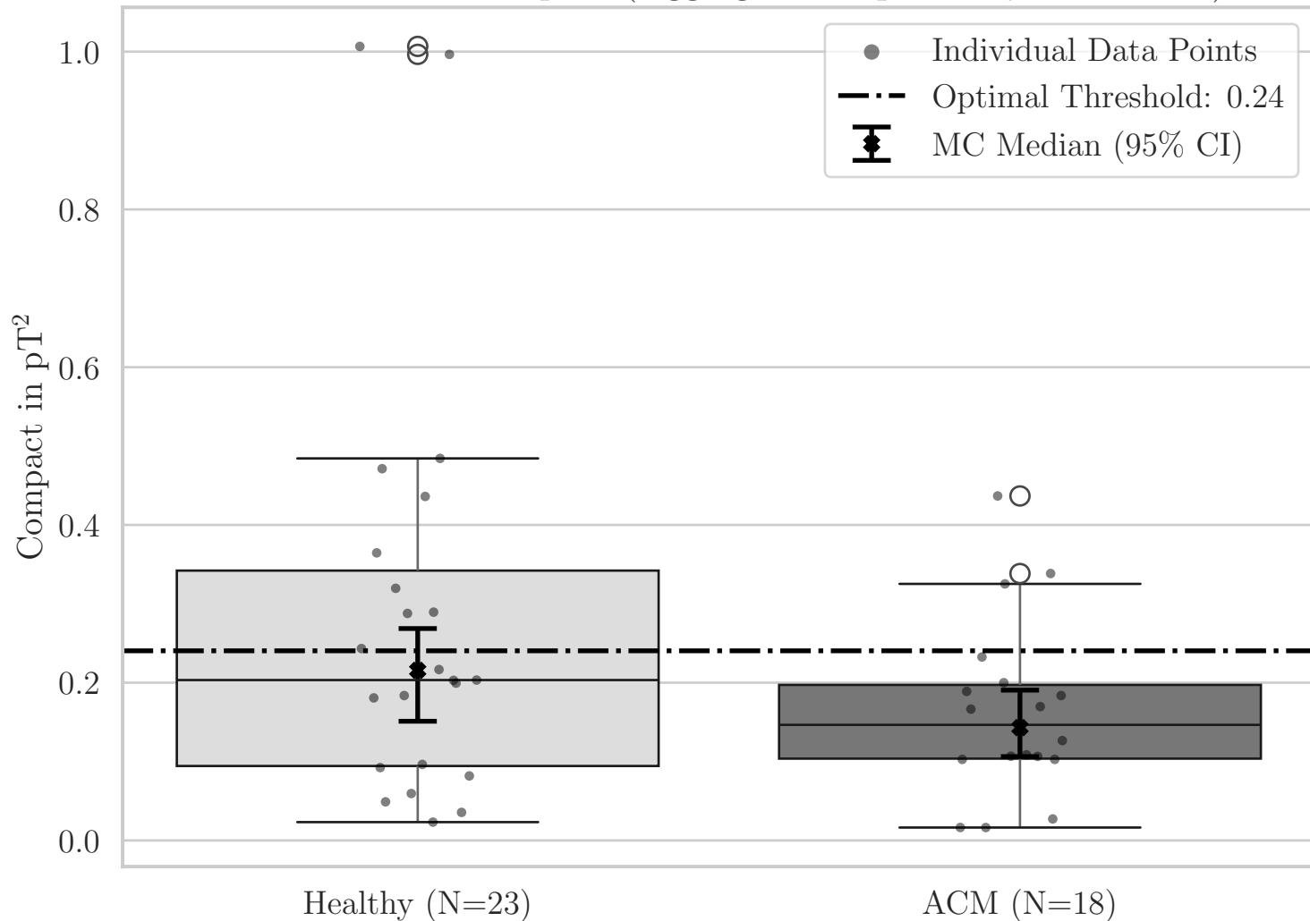
Box Plot for T Compact (Aggregated Top-Left Quadrant XY)
