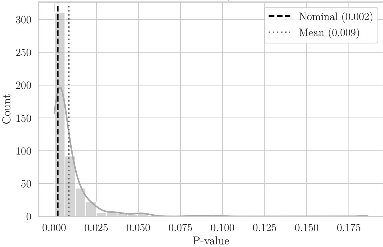
MC Distribution of P-values for T T-Dist (Aggregated Top-Left Quadrant XY)
